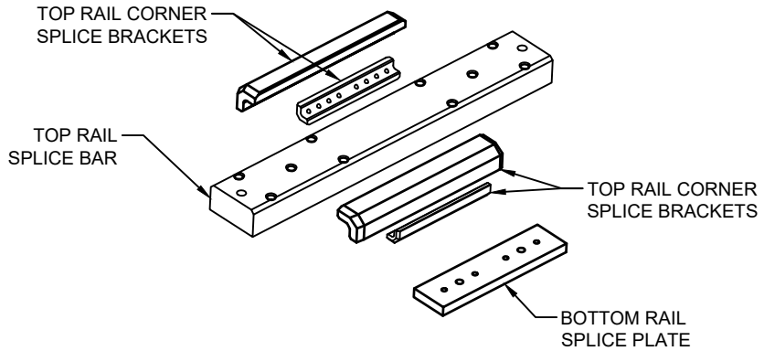
SPLICE KIT COMPONENTS SCALE: NTS
